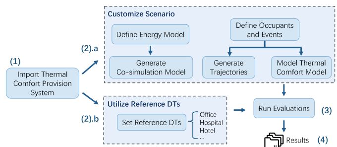
Fig. 2: Co-zyBench workflow.
