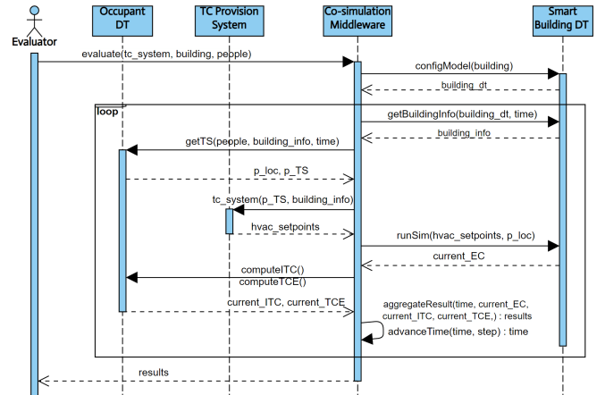
Fig. 5: Sequence diagram of Co-zyBench.
