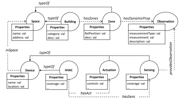
Fig. 3: The Smart Building-based NGSI-LD property graph.
