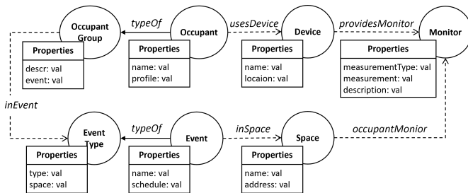
Fig. 4: The Occupant-based NGS-LD property graph.
