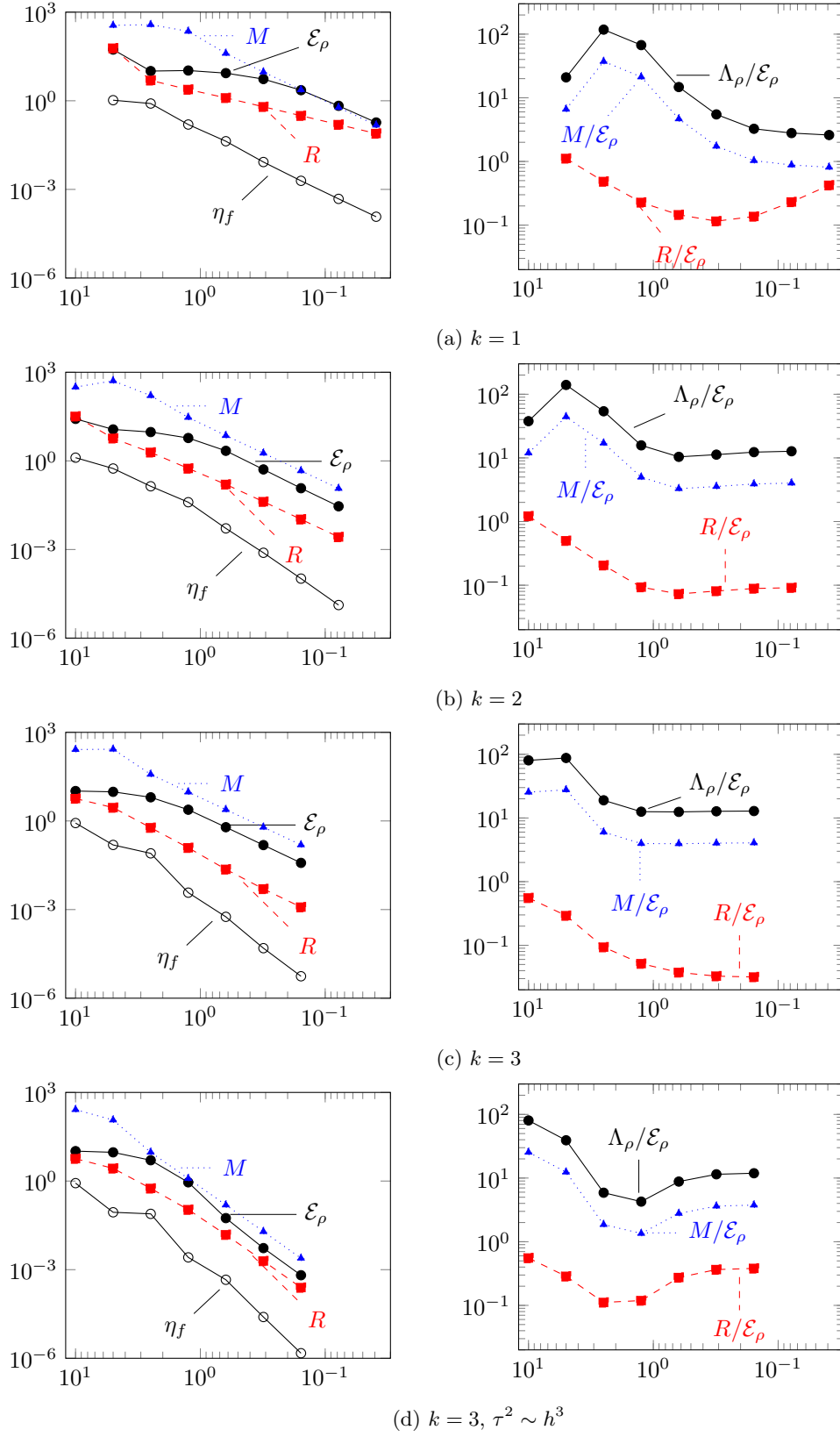
Figure 9: Propagating wave example with \rho = 0.01
