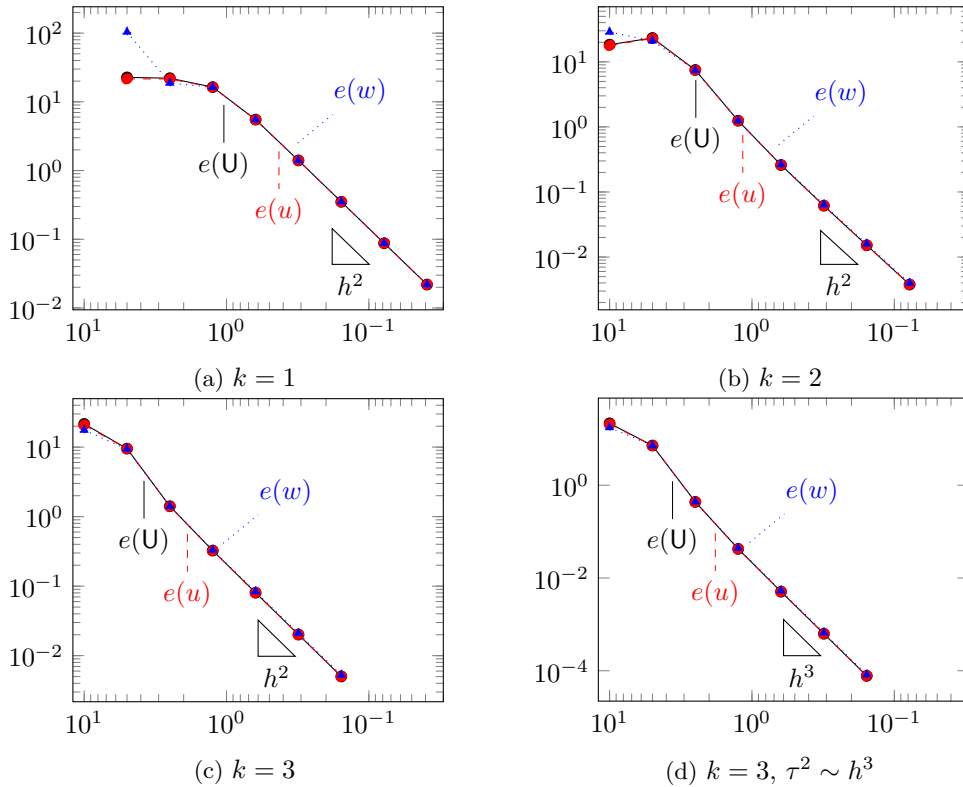
Figure 3: Standing wave: reconstruction errors on the solution
