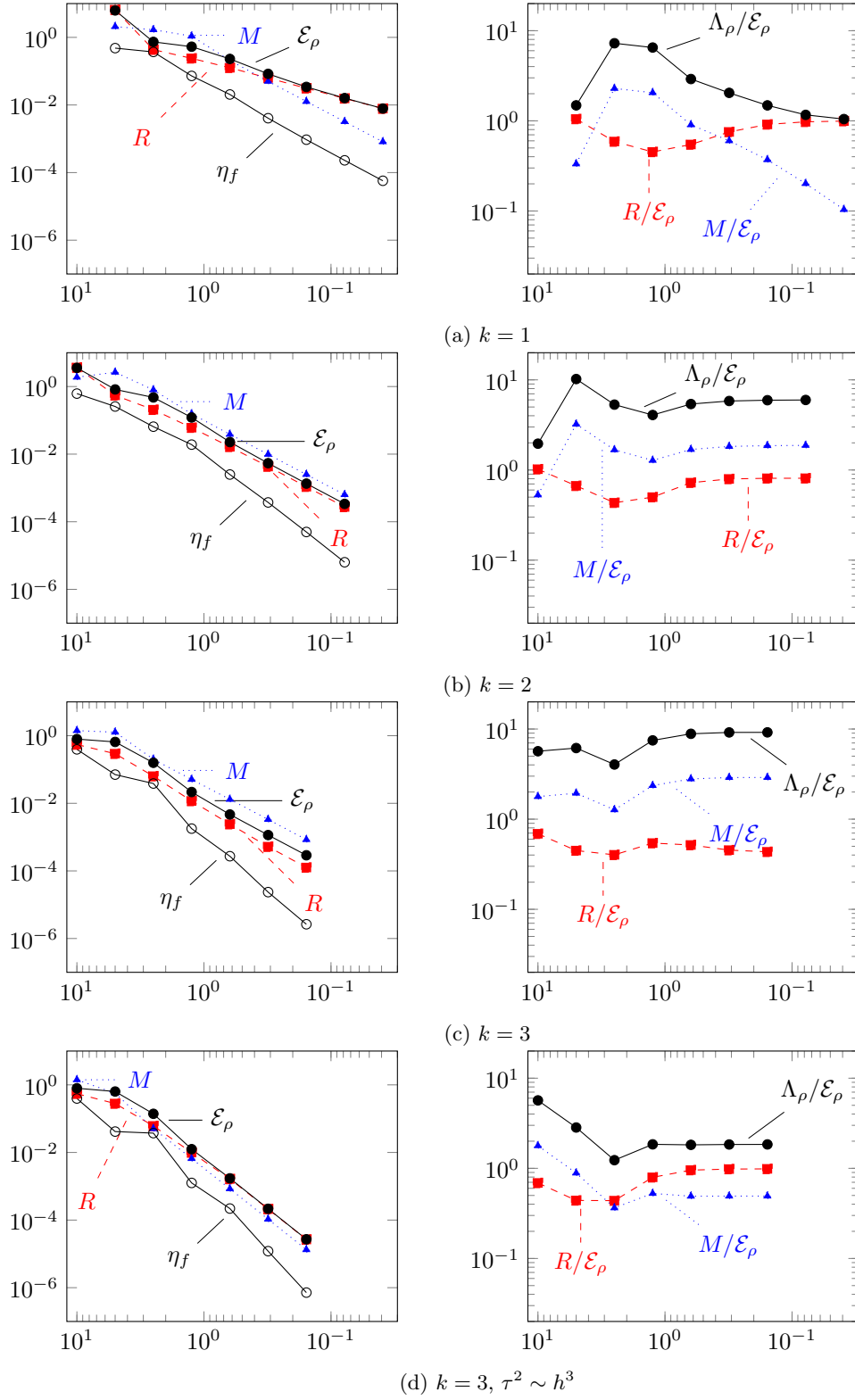
Figure 8: Propagating wave example with \rho = 0.2
