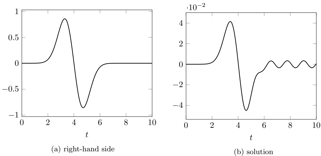
Figure 1: Time profiles in the standing wave example
