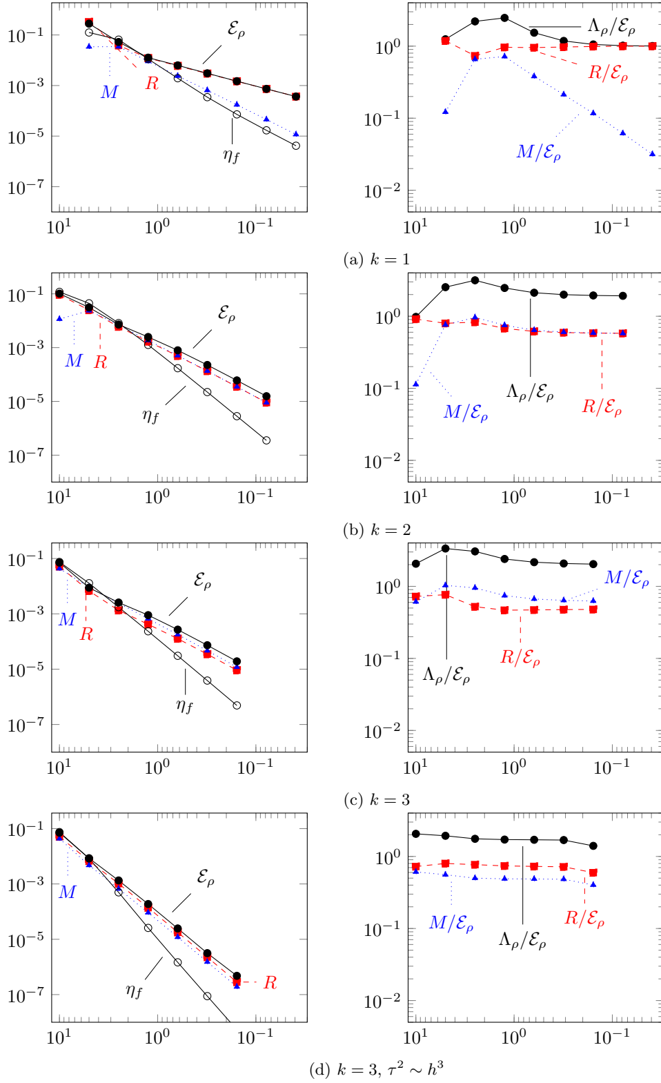
Figure 6: Standing wave example with \rho = 1
