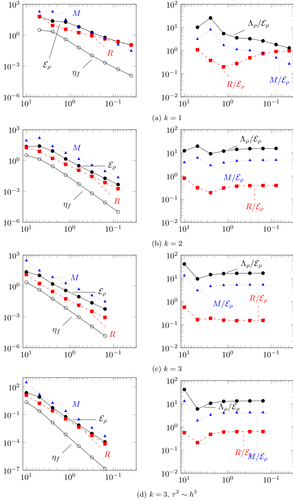
Figure 7: Standing wave example with \rho = 0.02
