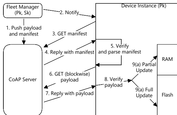
Fig. 5 Notification, fetching, verification and installation of model updates with RIOT-ML, securely over the network.
