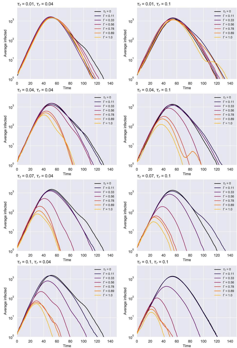
Fig 7. ER network—Epidemic evolution over time given a less efficient (left) and a more effective (right) testing regime. Results averaged over 105 simulations, obtained for N = 10000, K = 10, p_a = 0.2 . As the contact tracing rate increases, the accuracy of the network given by \Gamma becomes more important for “flattening” the curves. The case with no contact tracing ( \tau_t = 0 ) is colored in black.
