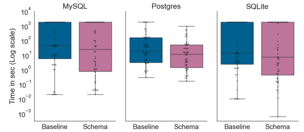
Figure 17: Query runtime on different RDBMS for LDBC.
