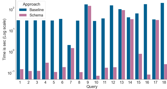
Figure 12: Query runtime for YAGO dataset.
