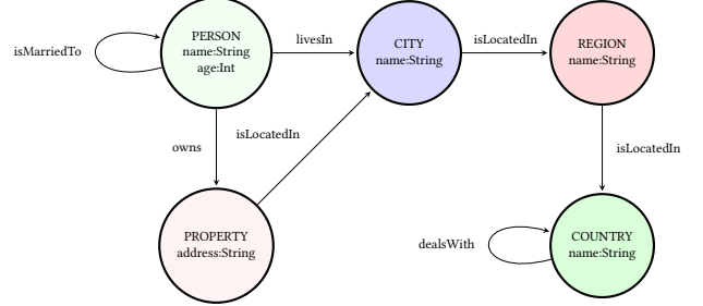
Figure 1: Sample graph schema for YAGO dataset.
