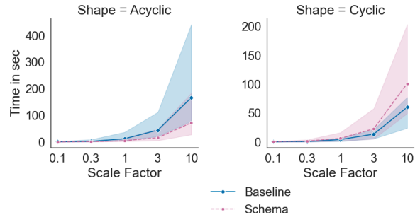
Figure 13: Runtime based on query shape.
