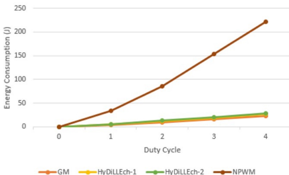
Figure 20. Cumulative energy consumption.
