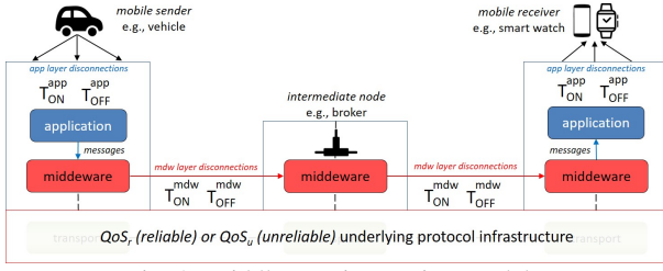
Fig. 2: Middleware interaction models.
