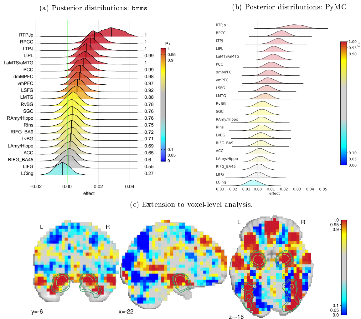
Figure 7: Validation of implementation using PyMC. (A) Posterior distributions of region-level behavior effects using brms . (B) Posterior distributions of region-level behavior effects using PyMC. (C) Posterior probabilities of the voxel-level effects being positive or negative, obtained using PyMC (plotted using Nilearn and overlaid in green with the NeuroQuery (Dockès et al., 2020) map for the term “emotional faces”).
