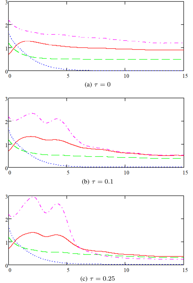
Figure 2: Behavior of |x(t)| + |z(t)| for different initial conditions and delays \tau , t \in [0, 15]
