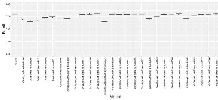
(b) Recall
