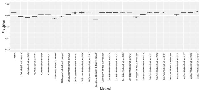
(c) Precision
