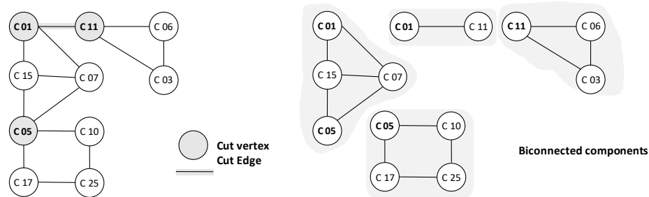
Fig. 4. Example of cut edge and cut vertex
