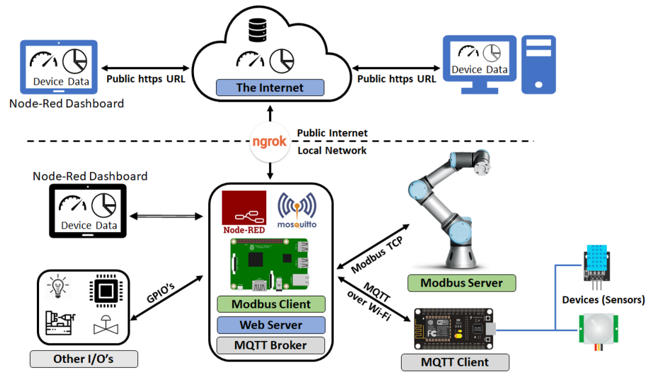
Fig. 4. Proposed architecture
