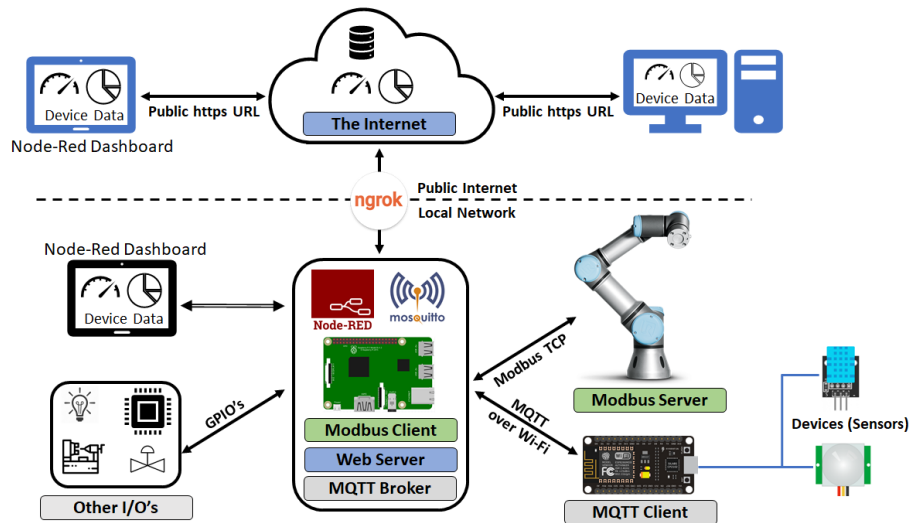
Fig. 4. Proposed architecture
