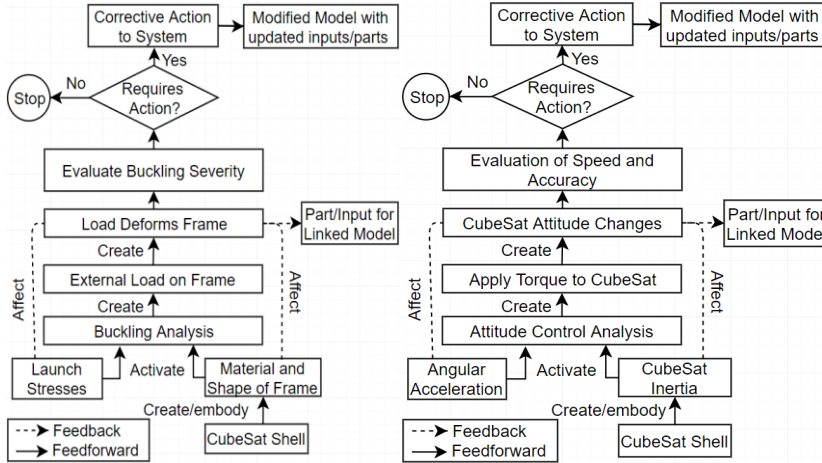
Fig. 3. Buckling Analysis
