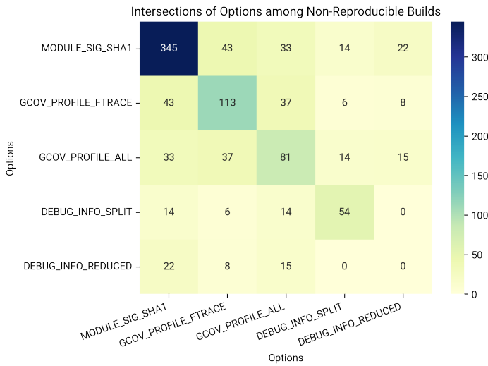
Figure 3: Intersections of Options from the Decision Tree
