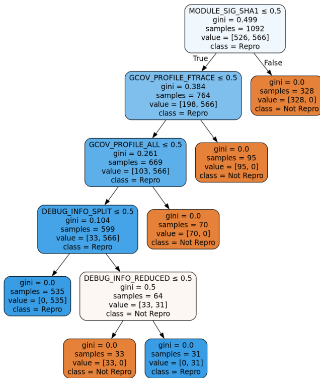
Figure 4: Decision tree obtained for Linux
