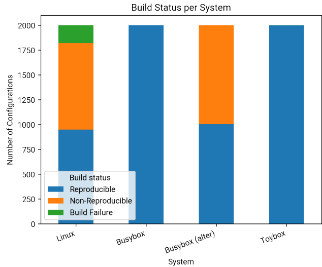
Figure 2: Build status per system
