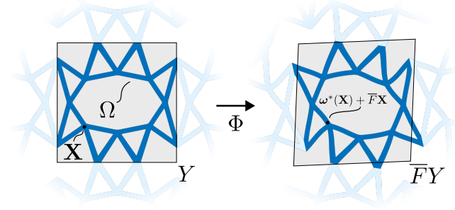
Fig. 3. We use nonlinear periodic homogenization to define the effective properties of a periodically tiled unit cell Y containing microstructure \Omega .
