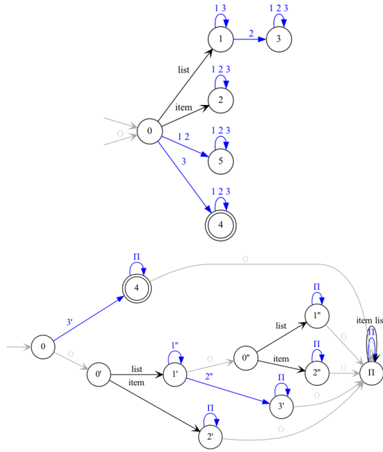
Figure 1. The unique minimal deterministic schema-complete SHA with initial state equal tree initial state for the XPath filter [self::list][child::item] .
