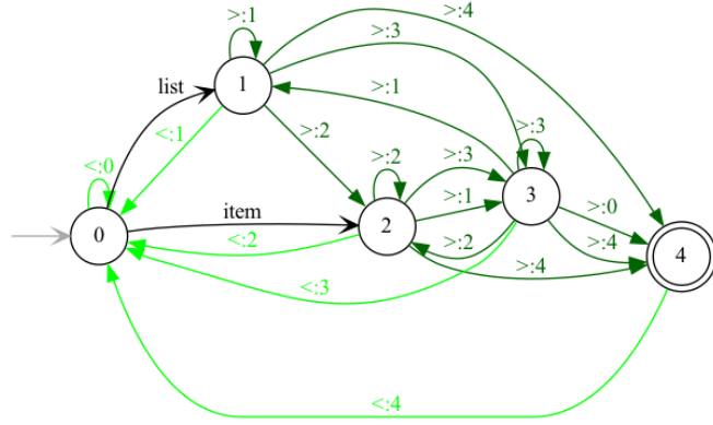
Figure 18. The dNWA A^{nwa} for the d\text{SHA}^\downarrow A in Fig. 7 obtained by applying the down operator to the d\text{SHA} in Fig. 1 for the filter [self::list] [child::item] .
