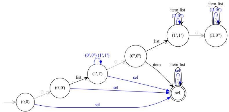
Figure 17. The earliest d\text{SHA} \downarrow A_{e(\mathbf{S})}^{\text{sncc}} with safe-no-change subhedge projection for the dSHA A in Fig. 1 with schema \mathbf{S} = \llbracket \text{doc} \rrbracket for the XPath filter [\text{self}::\text{list}] [\text{child}::\text{item}] .
