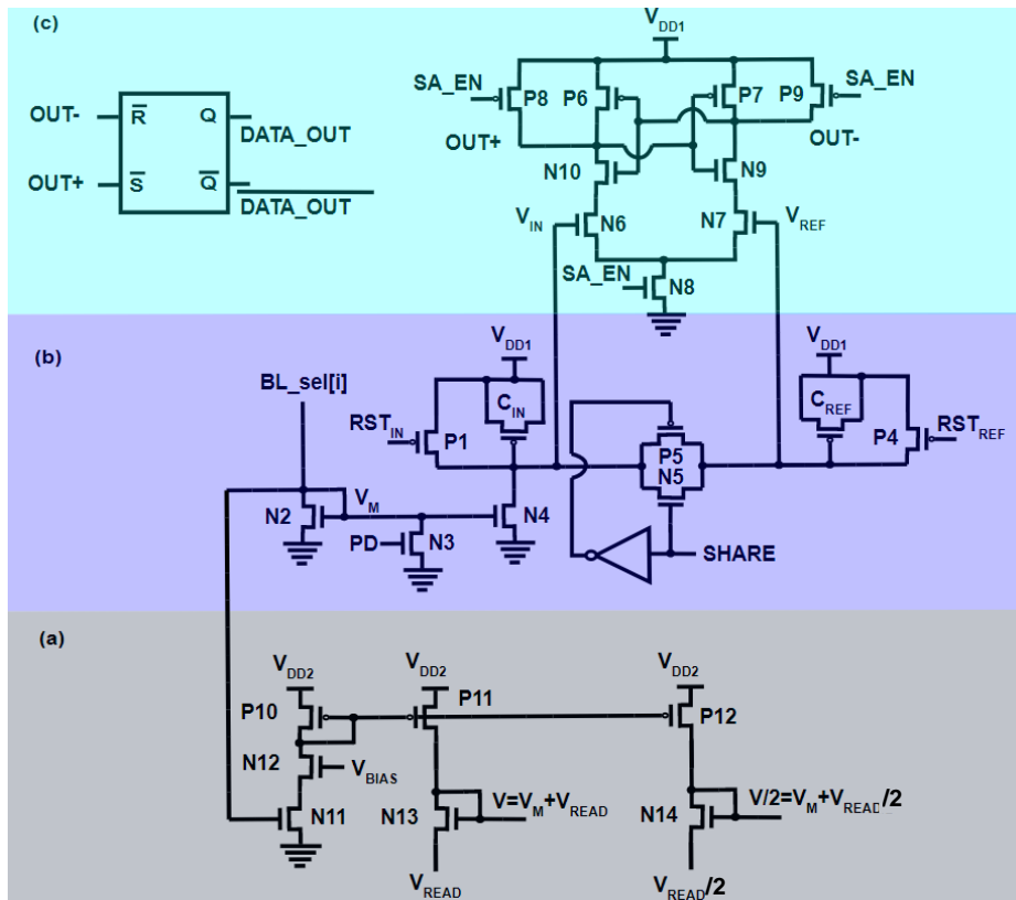
Fig. 3. Schematic of the proposed sense circuit with three main blocks: (a) the regulation block, (b) the capacitor block and (c) the comparator block
