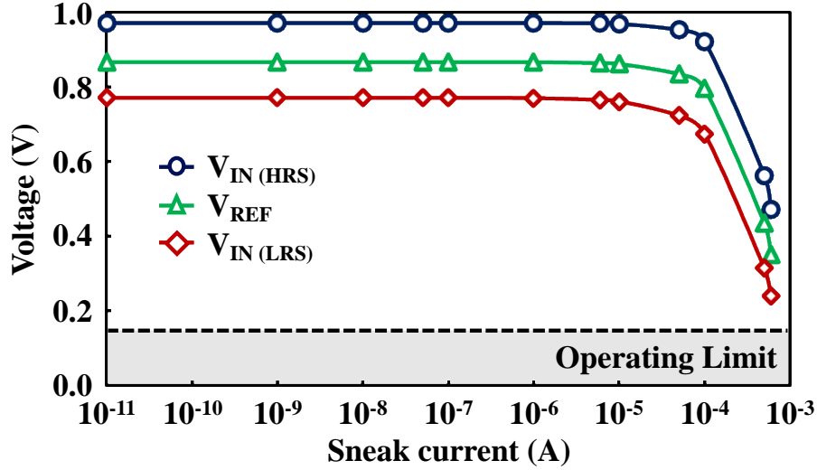
Fig. 7. Input voltage V_{IN} (corresponding to the read of a PCM HRS and respectively a PCM LRS) and voltage reference V_{REF} evolution versus the identified conditions given Table II for various OTS selector characteristic and array size.
