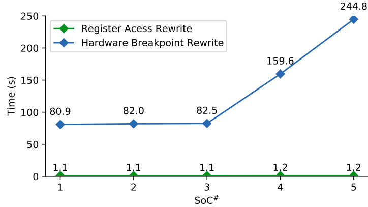
Fig. 9. Transformation time to apply rewrite rules. The hardware breakpoint rewrite rule introduces more design modifications when more hardware breakpoints are enabled. Whereas, the register access rewrite rule introduces the same design modifications in experimented SoCs.
