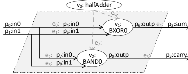
Fig. 2. Hierarchical port graph for a half adder. Solid black edges describe connections among ports and dashed grey edges depict hierarchizations of vertices (components).
