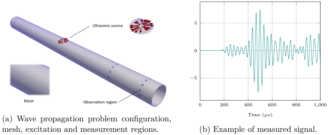
Figure 21: Configuration and examples of measured signals for the wave propagation problem. The measurement regions are represented in blue and the excited region in red.
