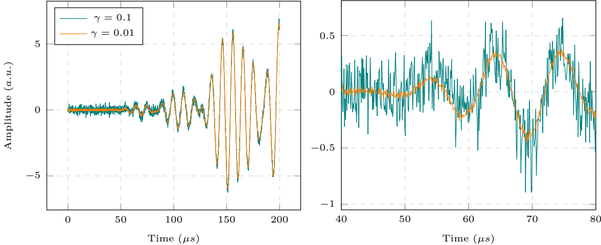
Figure 15: Example of different noise levels for the aluminum plate illustration.
