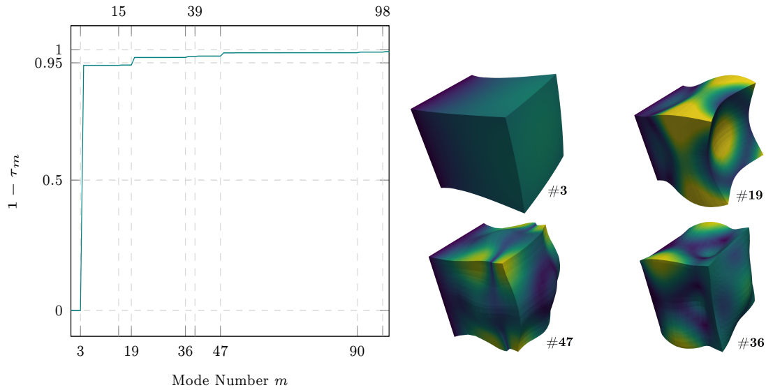
(a) Reconstruction error per number of modes. (b) Deformation associated with the relevant eigenmodes.
