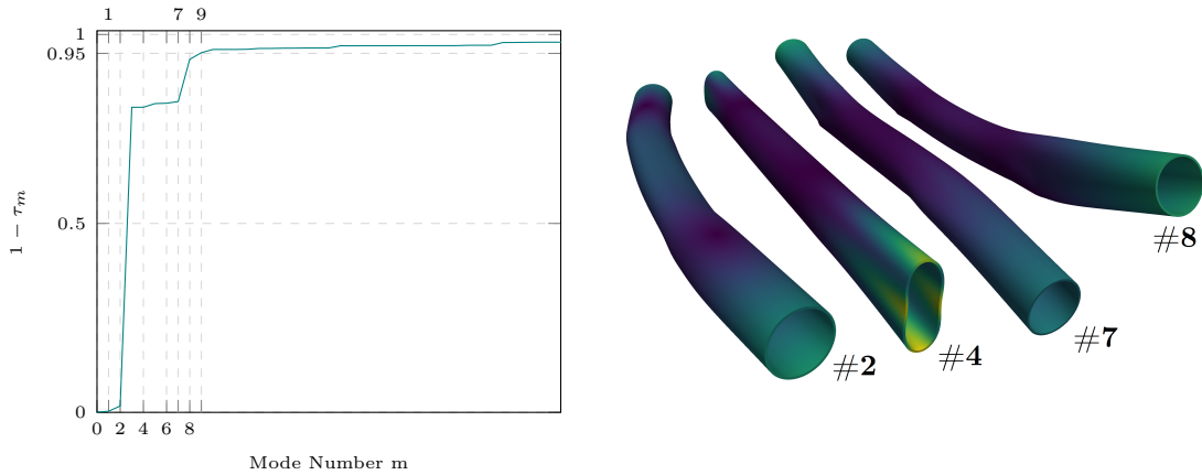
Figure 22: Reconstruction error of \mathbf{u}^* using the lowest frequency modes from which the selection of the most relevant modes is done.
