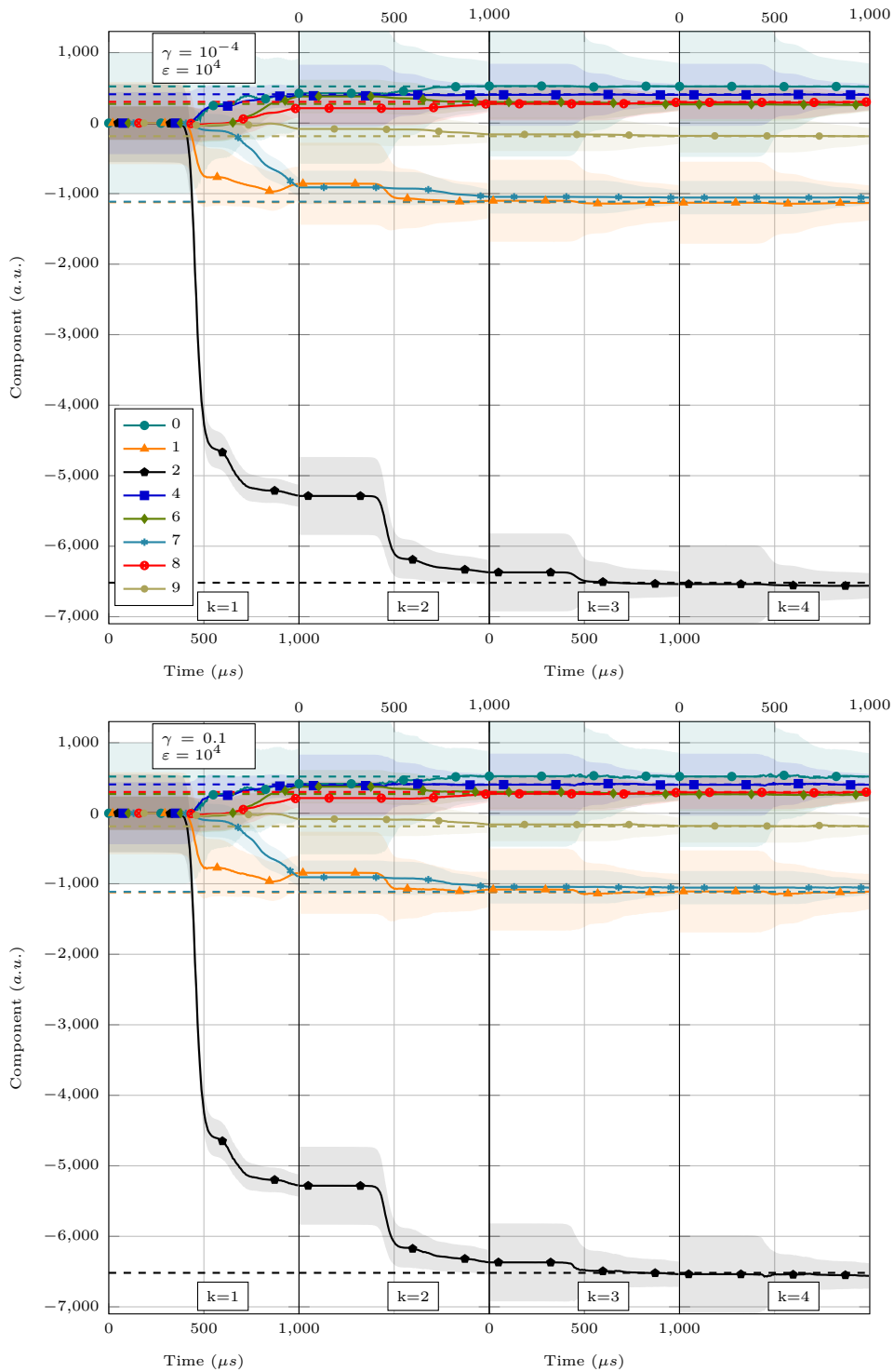
Figure 23: Evolution in time for the estimation \hat{\theta}_h^k for the pipe case. The estimated modes components are plotted with a highlighted region corresponding to the standard deviation. The target values are represented as dashed lines. Different \gamma noise levels are tested with a strong regularization \epsilon = 10^4 .
