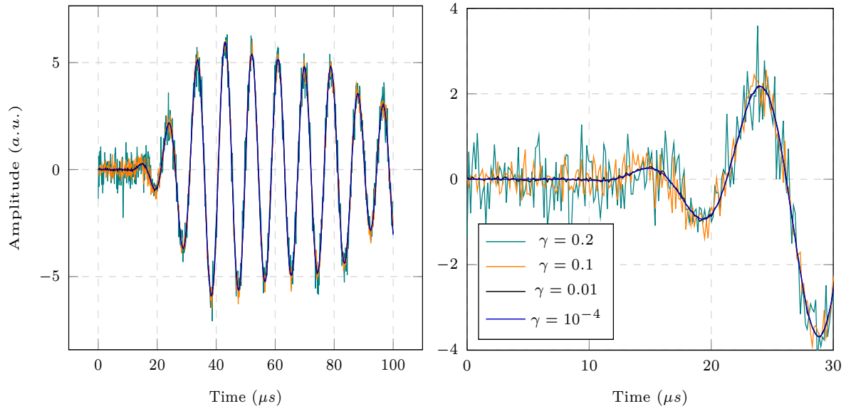
Figure 6: Example of different noise levels added to the synthetic data for the cube case.
