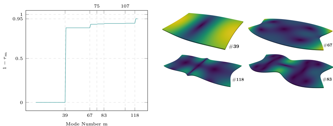
(b) Deformation associated with the relevant
