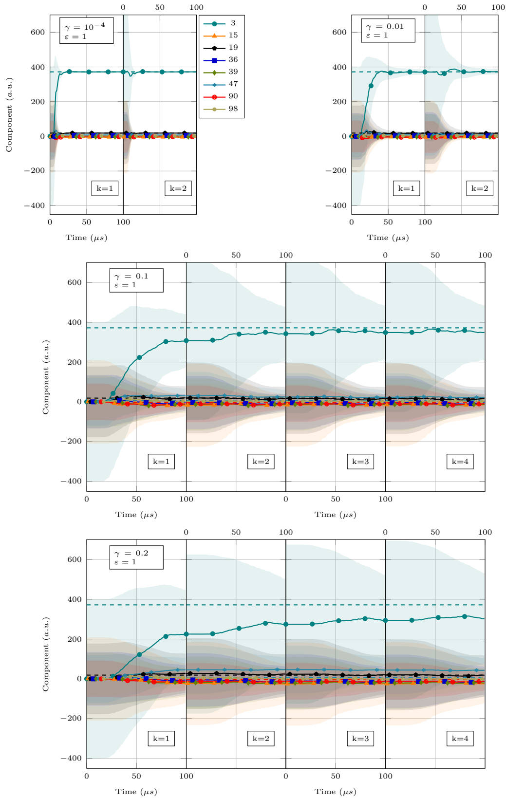
Figure 8: Evolution in time for the estimation \hat{\theta}_h^k for the cube case. The estimated modes components are plotted with a highlighted region corresponding to the standard deviation. The target values are represented as dashed lines. Different \gamma noise levels are tested with a regularization \varepsilon = 1 .
