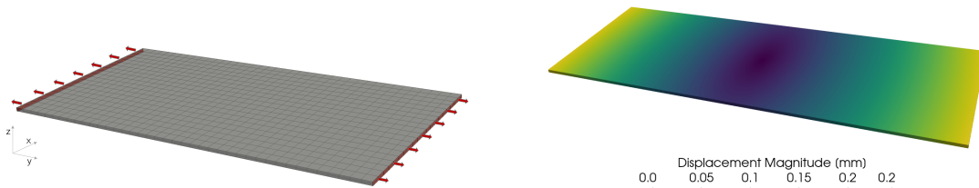
(b) Deformation for an axial stress of 57.5MPa.
