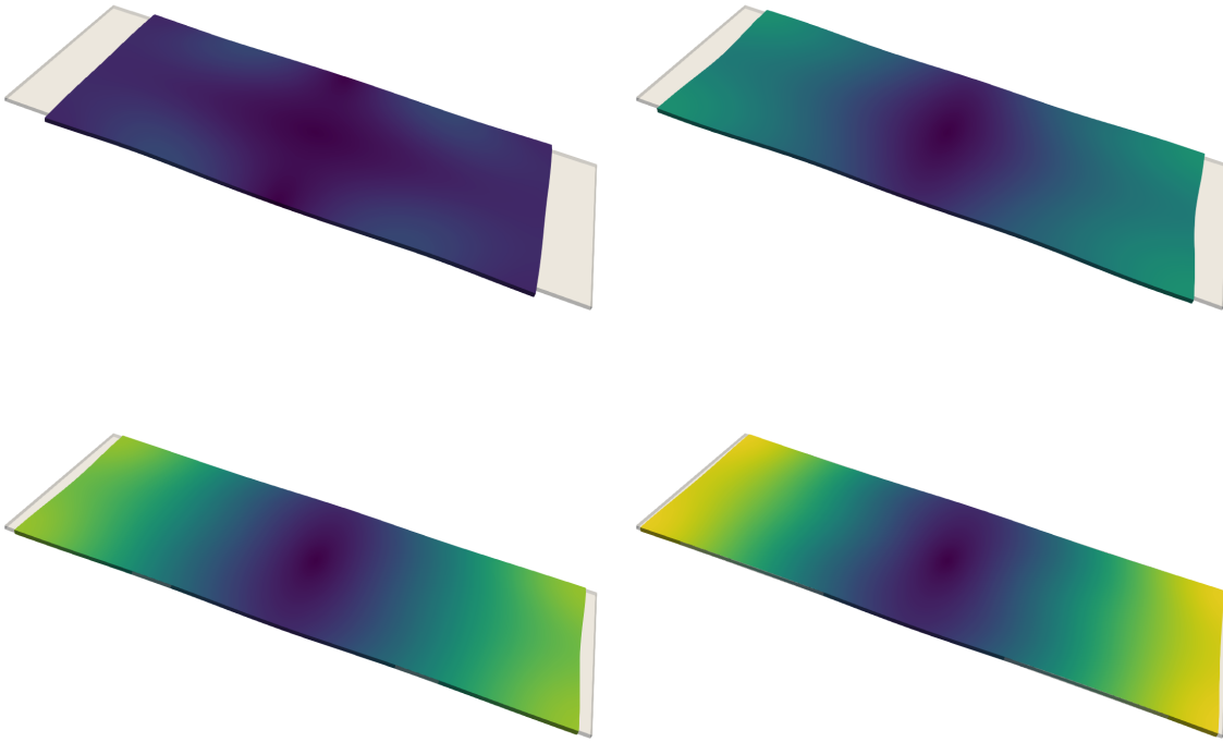
Figure 17: Snapshots at given iterations k and time t of the estimated deformation compared with the target deformation (transparent). Estimation for \gamma = 0.1 . From left to right, top to bottom we have (k=0, t=60\mu s) (k=0, t=130\mu s) (k=0, t=180\mu s) and (k=1, t=200\mu s) . Visualization is scaled 300x.
