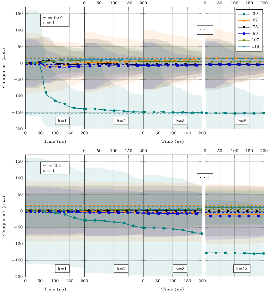
Figure 16: Evolution in time for the estimation \hat{\theta}_h^k for the plate case. The estimated modes components are plotted with a highlighted region corresponding to the standard deviation. The target values are represented as dashed lines. Different \gamma noise levels are tested with a neutral regularization \varepsilon = 1 .
