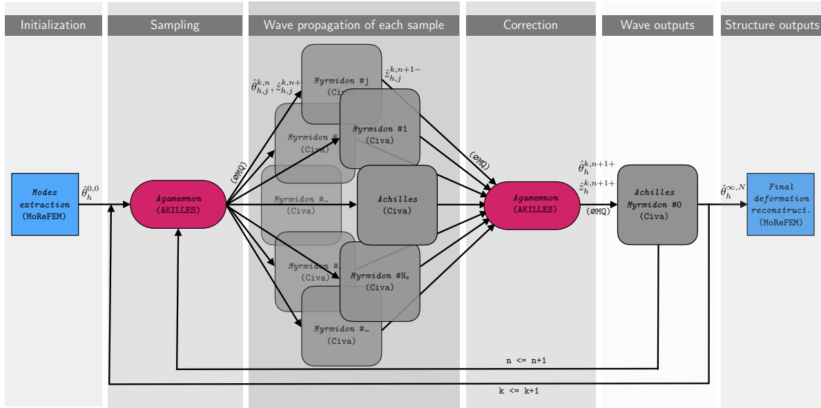
Figure 3: Parallel implementation of the DT-iROUKF in AKILLES.
