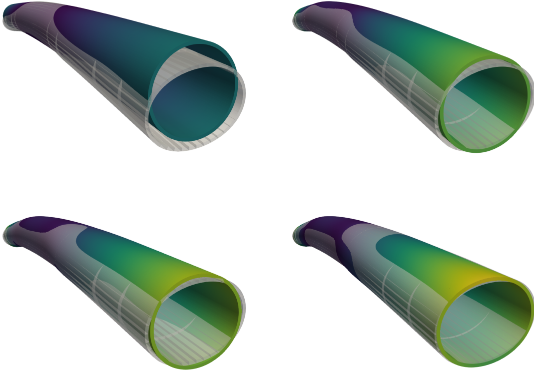
Figure 24: Snapshots at given iterations k and time t of the estimated deformation compared with the target deformation (transparent). Estimation for \gamma = 0.01 . From left to right, top to bottom we have (k=0, t=60\mu s) (k=0, t=130\mu s) (k=0, t=180\mu s) and (k=1, t=200\mu s) . Visualization is scaled 20x.
