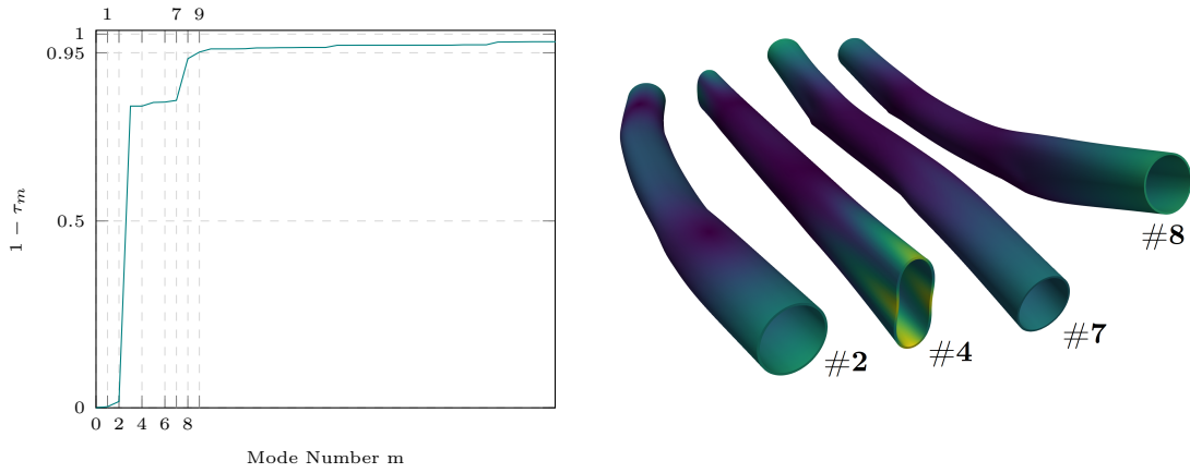
Figure 22: Reconstruction error of \mathbf{u}^* using the lowest frequency modes from which the selection of the most relevant modes is done.
