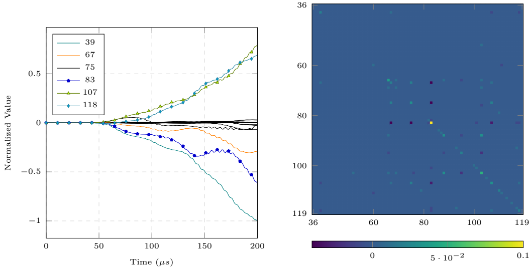
(c) Normalized Gramian at the end of the analysis.
