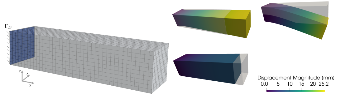
(a) Mesh and boundary conditions for the test
