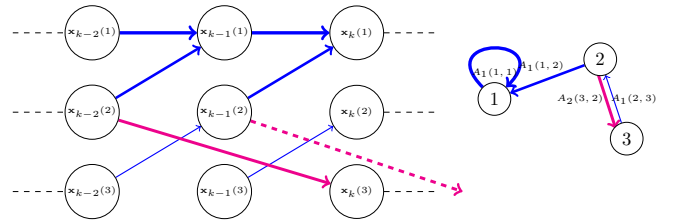
Fig. 1: Summary representation of the proposed graphical model, for the toy example. The edges in blue (resp. magenta) are defined as non-zero entries of \mathbf{A}_1^\top (resp. \mathbf{A}_2^\top ). Edge thickness is proportional to the absolute entries of these matrices. Left: Dynamic state evolution. Right: Graphs associated to matrices \mathbf{A}_1 and \mathbf{A}_2 .
