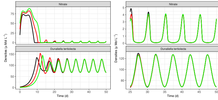
(B) Dynamics with \tau = 1.2 d .
