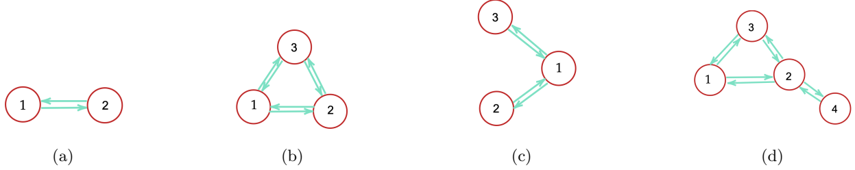
Figure 1: For the purpose of visualization , the international system can be represented as a graph capturing the hostility relationships between the Nations. Formally, n is an opponent of m if and only if m \in \sigma(n) , which materializes through the existence of an oriented edge linking n \rightarrow m . In 1a and 1b , the international system is represented as a complete graph involving two and three Nations respectively. In 1c the graph is semi-bipartite , whereas in 1d , the graph has two cliques capturing local-global interactions.
