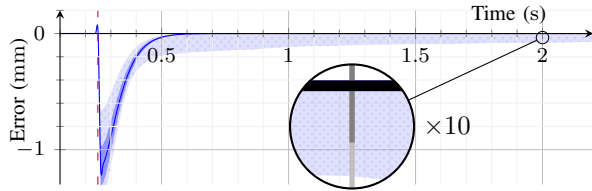
Fig. 2: Error profile (solid blue) of the deviation norm \|\hat{e}\| - \|\epsilon_s\| , for all tested configurations with both -20 N and 20 N simulated force inputs on the \vec{x} axis. The interquartile range is coloured in blue, while the light blue dotted area represents 90% of the data between the 5% and 95% percentiles. Zoom ratios are indicated next to the zoomed windows. The force input starting front is signified with the vertical dashed purple line.
