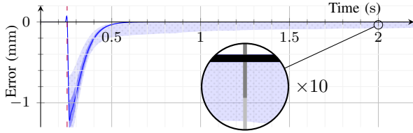
Fig. 2: Error profile (solid blue) of the deviation norm \|\dot{\epsilon}\| - \|\epsilon_s\| , for all tested configurations with both -20\text{ N} and 20\text{ N} simulated force inputs on the \vec{x} axis. The interquartile range is coloured in blue, while the light blue dotted area represents 90 % of the data between the 5 % and 95 % percentiles. Zoom ratios are indicated next to the zoomed windows. The force input starting front is signified with the vertical dashed purple line.
