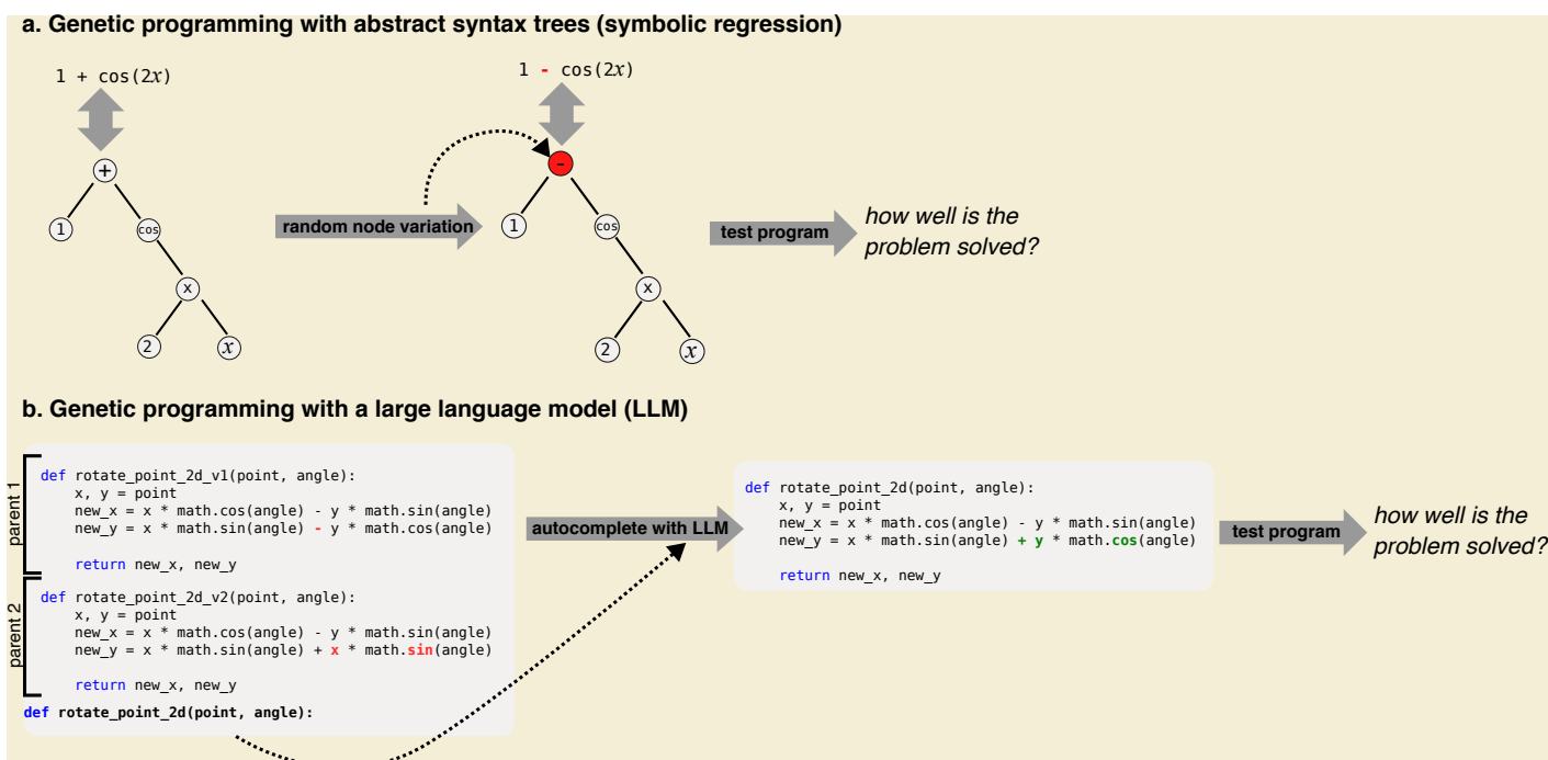
Fig. 1. Genetic programming with large language models. a , Genetic programming is a computer-science approach that ‘mutates’ code, one variation at a time. When a computer program can be represented with an abstract ‘tree’ structure, then genetic programming involves changing one node in the tree at random, testing to see if the change has improved the program, and then repeating the process on the highest-performing programs. b , Instead of making changes to an abstract tree, Romera-Paredes et al. 3 devised a genetic programming method that involves taking two programs, concatenating them, and asking a large language model (LLM) to generate a third program by autocompleting the concatenated pair. This approach enabled the authors to generate new variants of programs that are likely to be meaningful in their context.
