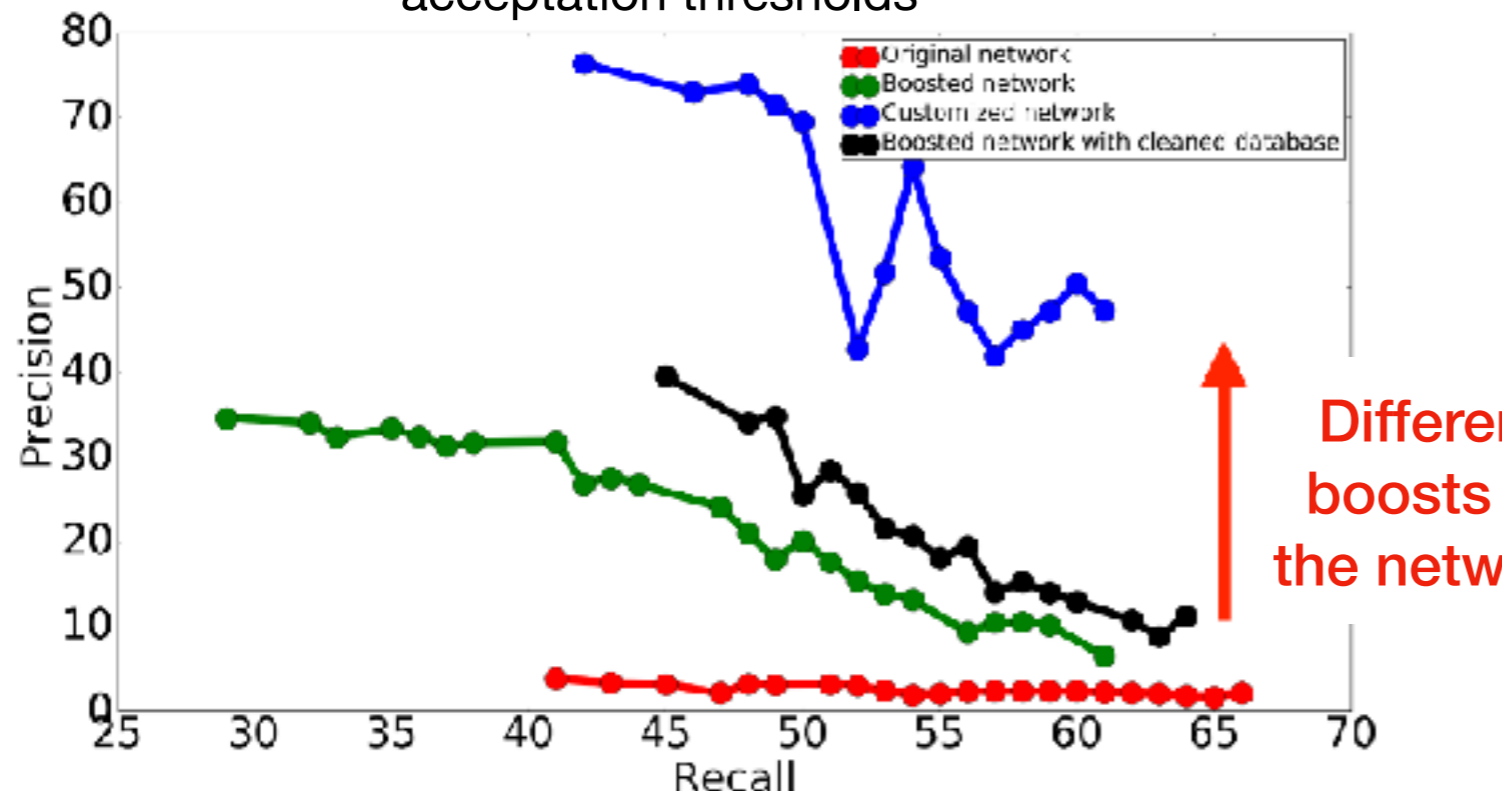
ROC curve: precision vs recall for different acceptance thresholds
