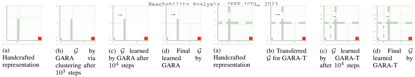
Fig. 4: Goal space representations for the 4-Rooms Maze
