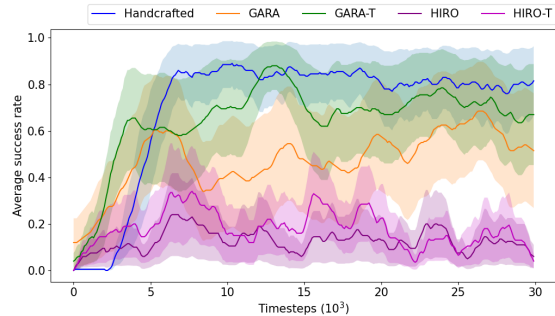
Fig. 5: Average success rate on the 4-Rooms Maze (over 20 runs). -T refers to the transferred versions of the algorithms.
