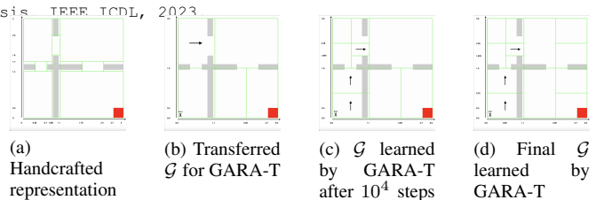
Fig. 4: Goal space representations for the 4-Rooms Maze
