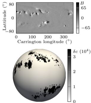
(b) Active region as velocity perturbation
