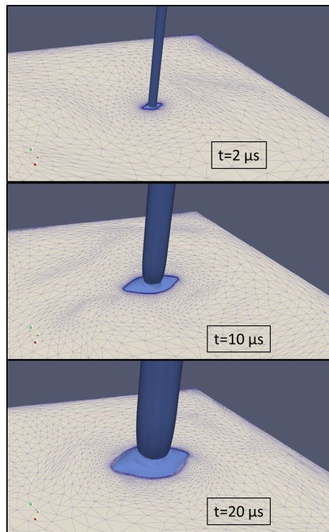
Figure 4: 3D plots of isocontours value at T = 5\,000 \text{ K} at times t=2 \mu\text{s} , 10 \mu\text{s} and 20 \mu\text{s} are shown.
