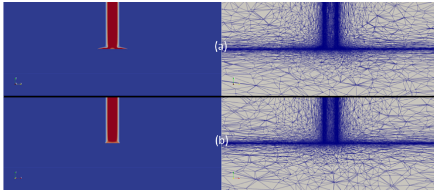
Figure 5: 2D plots of temperature distributions and mesh at times t = 2 \mu\text{s} . 2D cuts along the y direction "(a)" and along the x direction "(b)"
