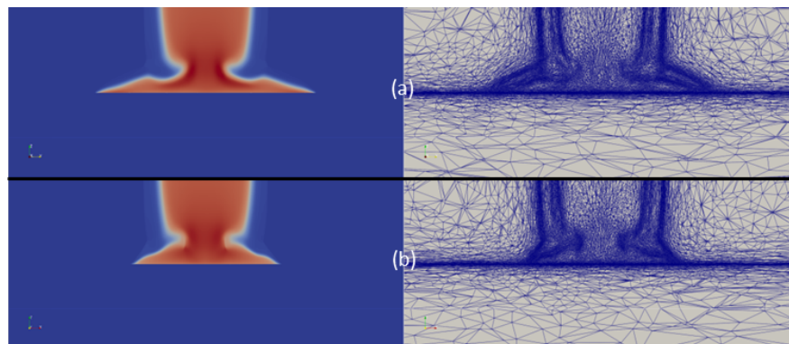
Figure 7: 2D plots of temperature distributions and mesh at times t = 20 \mu\text{s} . 2D cuts along the y direction "(a)" and along the x direction "(b)"
