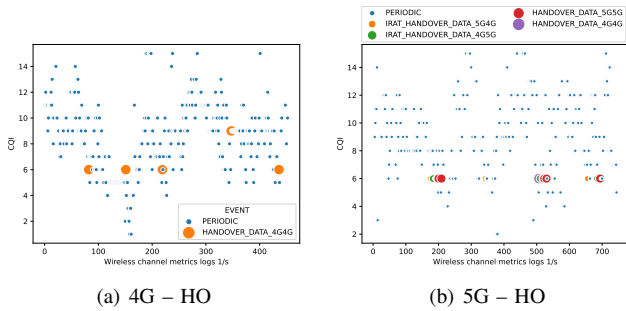
Fig. 7: 4G vs. 5G HO and CQI impact.
