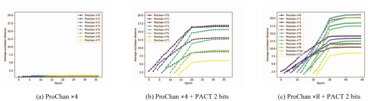
Figure 3: The euclidean difference between inputs and outputs of every ProChan module, for three different training setups, averaged on all the ImageNet validation set. The y-axes were set to highlight the difference in magnitude. pressed in 8 bits (weights and activations), but in a mixed precision setup, further reducing memory costs by adding PACT 2 bits on already compressed activations will only cost a 1% drop in Top1. However for bigger ProChan compression like \times 8 , the damages from PACT are amplified.
