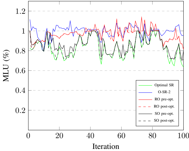
Fig. 5: MLU comparison on BtEur. ( |V| = 24, |A| = 74 ) with 10% variation
