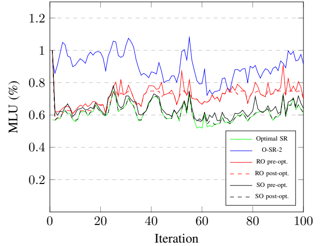
Fig. 6: MLU comparison on Hurri. ( |V| = 24, |A| = 74 ) with 10% variation
