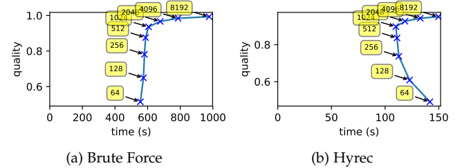
Fig. 7. Relation between the execution time and the quality in function of the size of SHF.
