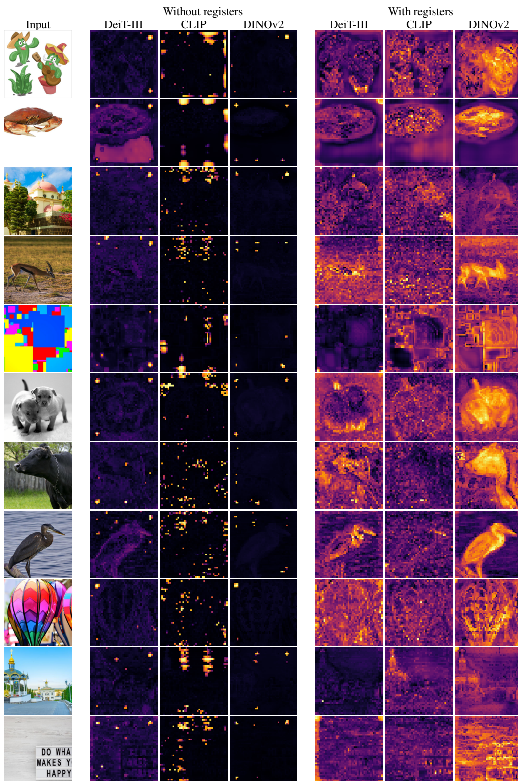
Figure 16: Norm the feature maps output by models trained without and with registers on various images. The norm outliers are very visible for models trained without registers.
