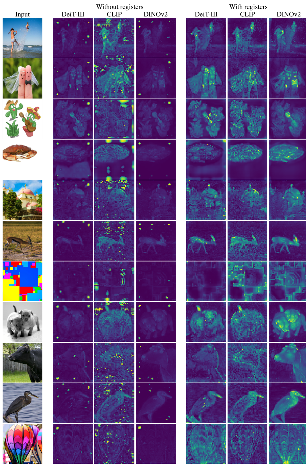
Figure 14: Attention maps of models trained without and with registers on various images.
