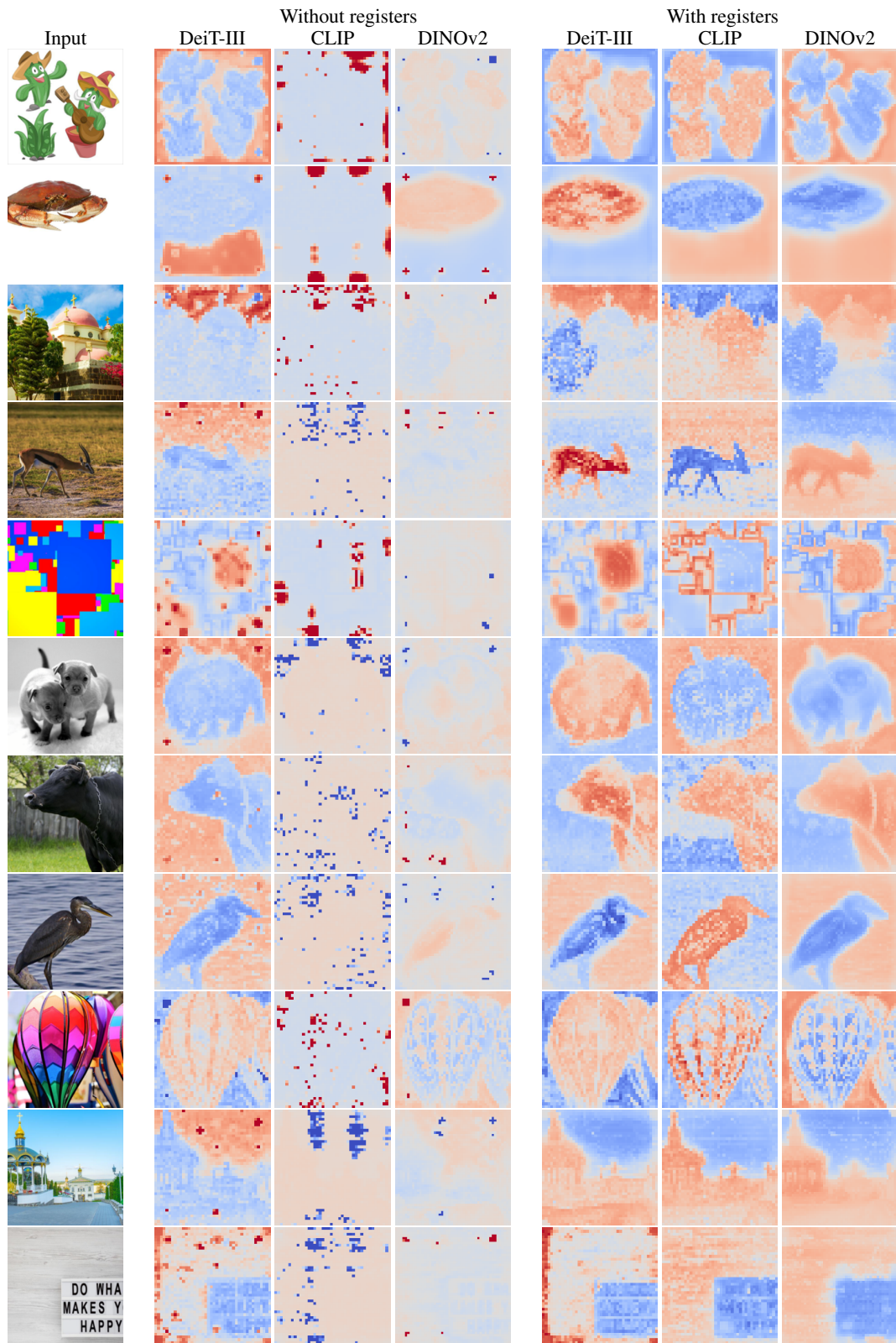
Figure 15: First principal component of the feature maps output by models trained without and with registers on various images. The components are whitened and the colormap covers the range [-3\sigma, +3\sigma] .
