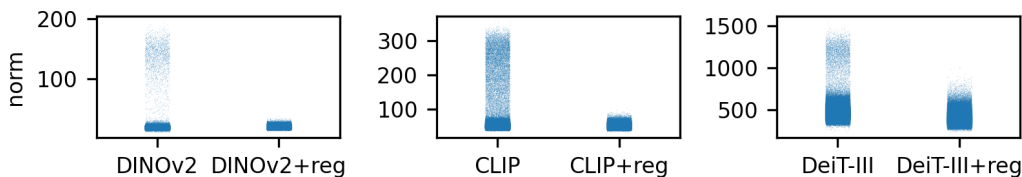
Figure 7: Effect of register tokens on the distribution of output norms on DINOv2, CLIP and DeiT-III. Using register tokens effectively removes the norm outliers that were present previously.
