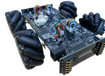
Figure 1: Current Version of the FreeBot with Mecanum Wheels and Front/Rear charging ports (152x133x48mm)
