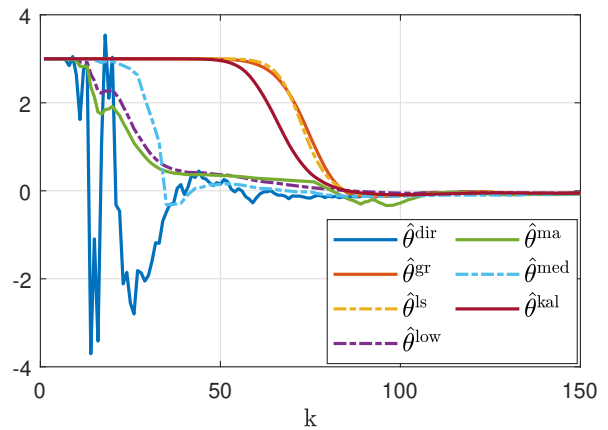
Fig. 2. Estimation error transients for noisy measurements: the direct estimation \hat{\theta}^{\text{dir}} (11), the gradient estimator \hat{\theta}^{\text{gr}} (12), the least-squares estimator \hat{\theta}^{\text{ls}} (13), the low-pass filtering \hat{\theta}^{\text{low}} (14), the moving-average filtering \hat{\theta}^{\text{ma}} (15), the median filtering \hat{\theta}^{\text{med}} (16), the Kalman filter \hat{\theta}^{\text{kal}} (17).
