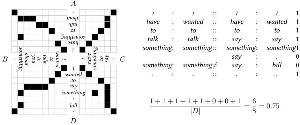
Figure 1: Computation of analogical score. Black cells in matrices indicate alignment points between tokens. Each token quadruple linked by alignments, one for each (sub-)word in D , is checked for trivial analogy. We divide by the length of D to get the analogical score. If A : B :: C : D is a strict analogy, the score is 1.
