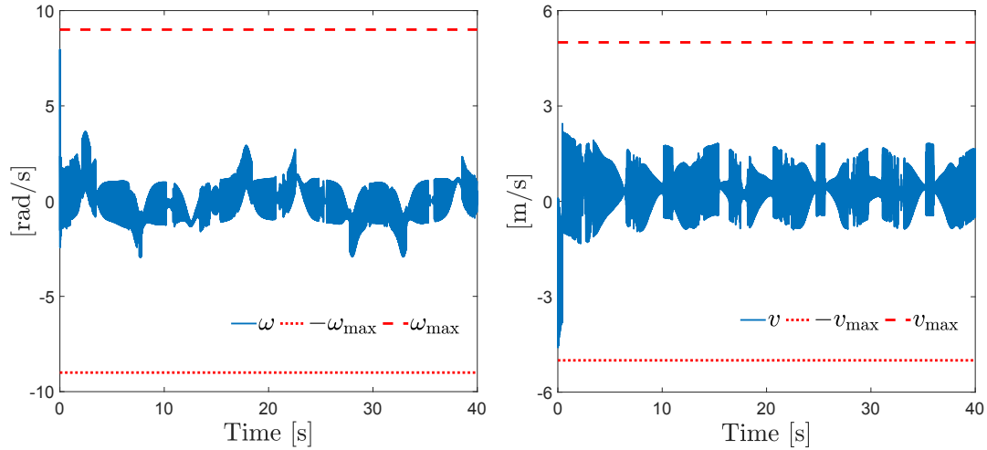
Figure 2. Control Signals
