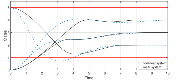
Fig. 1. Trajectories of the system states x_{i1} subject to the linear and nonlinear control protocols (disturbance-free case)
