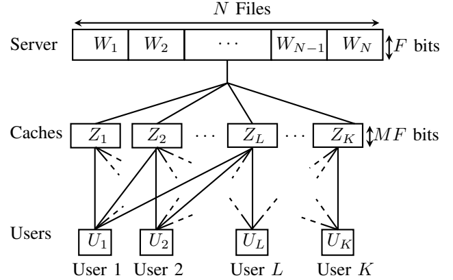
Fig. 1. The (N, K, L) multi-access cache network
