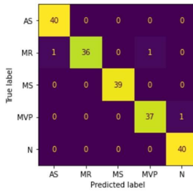
Fig. 9. Confusion matrix for Fold 6
