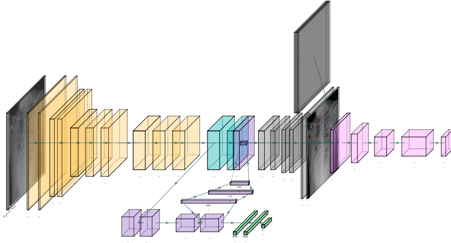
Fig. 3. Auto-Annotation GAN can colorize the tubular structures of catheters in CXR’s based on different classes, It is a combination of Discriminator Network, D_{\Lambda} in pink, and the Generator Network, G_{\Psi} which consist of two-subnets: G_{\Psi_1}^1 (yellow, aqua-green, purple and gray layers) and G_{\Psi_2}^2 (yellow, purple and gray layers).
