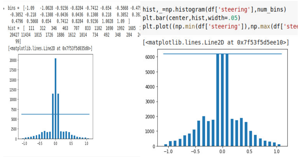
Fig. 3. Histogram of steering angle-1
