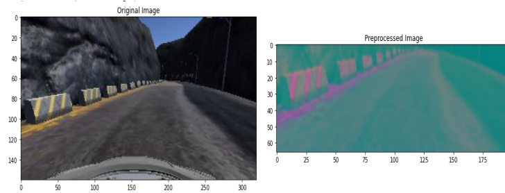
Fig. 9. Pre-processed image
