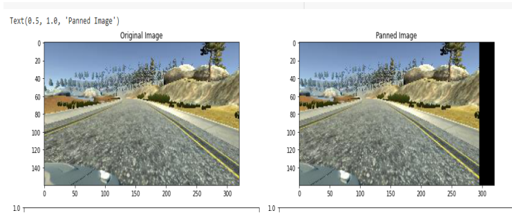
Fig. 7. Panned Image
