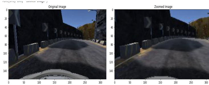
Fig. 5. Zoomed Image
