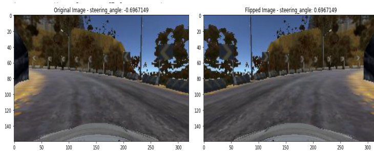
Fig. 8. Flipped Image
