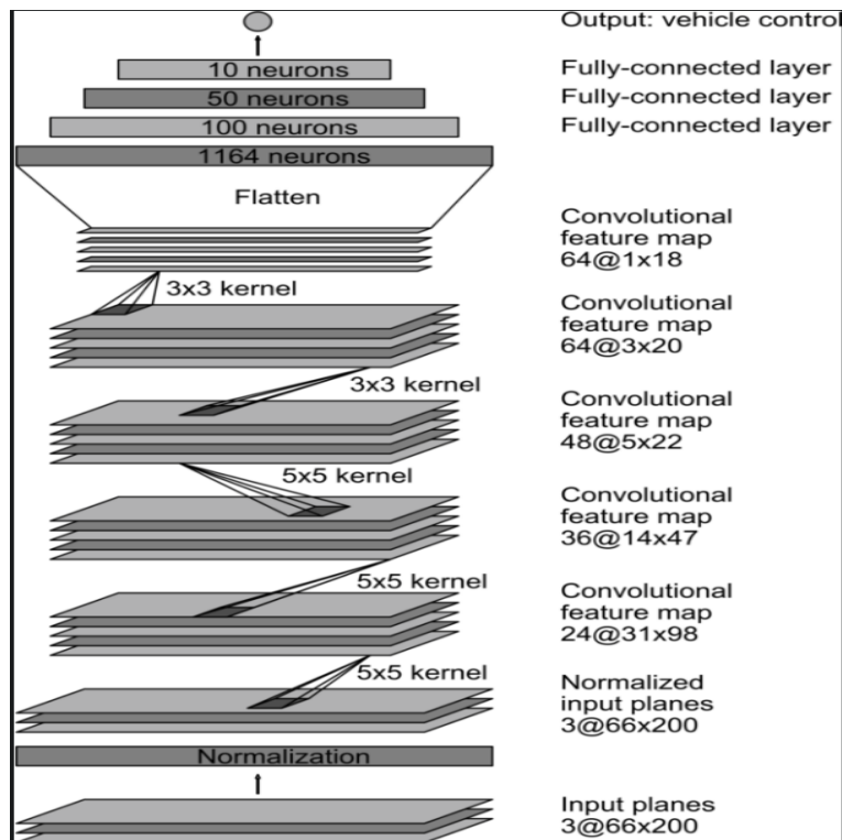
Fig. 13. Architecture
