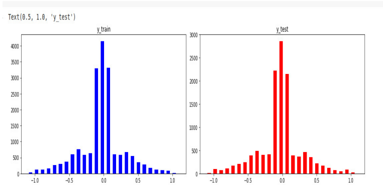
Fig. 12. Histogram Distribution of steering angles after train-test split
