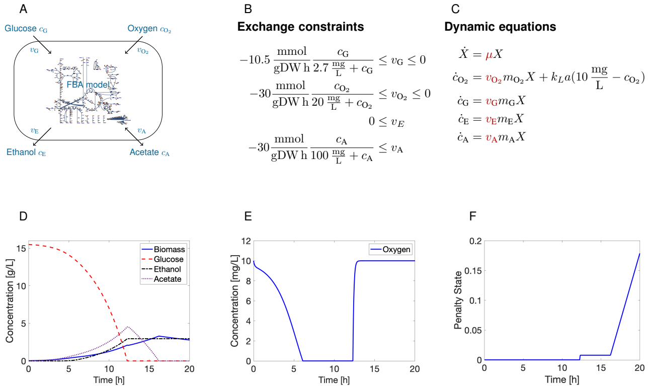
Figure 10.4: Example result of a DFBA simulation for the E. coli core model [98] performed with DFBAlab. A : Illustration of dynamic metabolites and relevant exchange fluxes. Extracellular metabolites use mass concentration (g/L), exchange fluxes are in molar amount per dry biomass and time (mmol/gDW h). B : Concentration-dependent constraints applied to the exchange fluxes during the DFBA simulation. C : Differential equation model for biomass concentration X and metabolite mass concentrations. Growth rate \mu and exchange fluxes v_* (in red) are optimal values from the underlying FBA model. m_{O_2} , m_G , m_E , m_A are molar masses of O_2 , glucose, ethanol, and acetate, respectively. k_L a = 8.5 \text{ h}^{-1} is the volumetric mass transfer coefficient for oxygen. D : Simulation results for concentrations of biomass and metabolites. We can observe four growth phases: aerobic growth on glucose with production of acetate, anaerobic growth on glucose with production of ethanol and acetate, aerobic growth on acetate, and a stationary phase. E : Simulation result for oxygen concentration in the liquid medium. Oxygen is depleted in the second growth phase due to mass transfer limitations, but replenishes at the start of the third phase. F : Penalty function time course. Increases of the penalty function indicate periods where the underlying FBA model is infeasible. Here, this occurs when the ATP maintenance constraint cannot be satisfied due to a lack of substrates, and happens in this simulation during a brief period where the switch from glucose to acetate as a substrate takes place, since oxygen needs to be replenished first, and in the stationary phase.
