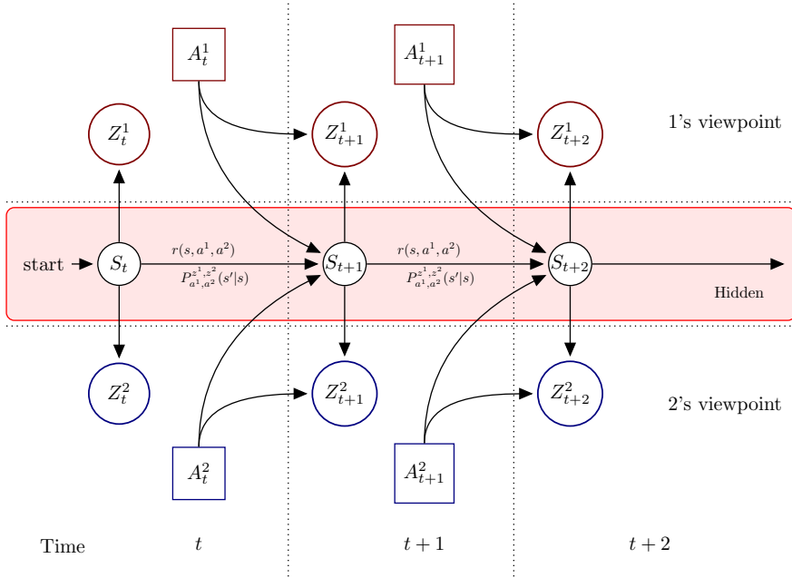
Fig. 1 Dynamic influence diagram representing the evolution of a zs-POSG
