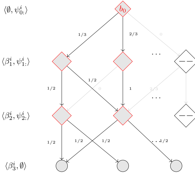
Fig. 3 Representation of the strategy recursively induced by some \psi_0^1 . At each time step \tau , one must (i) sample a next tuple/node w_\tau^1 from current distribution \psi_\tau^1 , (ii) apply DR \beta_\tau^1[w_\tau^1] , and (iii) make \psi_{\tau+1}^1[w_\tau^1] the new current distribution (unless reaching a leaf).
