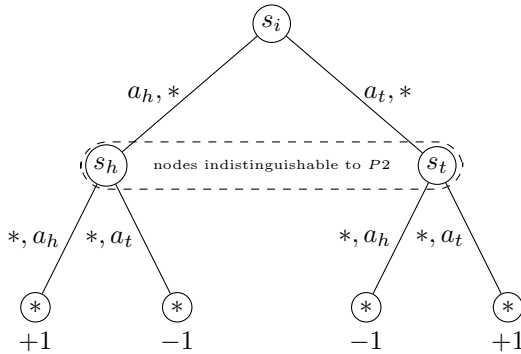
Fig. 2 Simplified tree representation of the sequentialized Matching Pennies game. Irrelevant actions, noted *, allow merging edges with the same action for (i) player 2 at t = 0 , and (ii) player 1 at t = 1 . Notes: (a) Due to irrelevant actions, this game can be seen as an Extensive Form Game, despite players acting simultaneously. (b) Players only know about their past action history (in this observation-free game).
