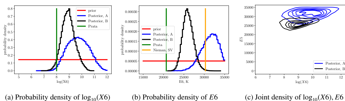
Figure 2: Probability densities of the efficiency and the activation energy of reaction 6. Blue histograms refer to the parameters posterior using set A, black histograms using set B, red lines indicate the prior distributions, green lines the values obtained by Prata et al., and yellow lines the theoretical values obtained by Nieman et al.
