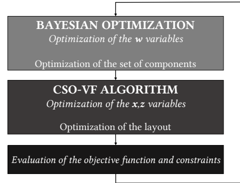
Figure 1: Structure of the two-level algorithm.
